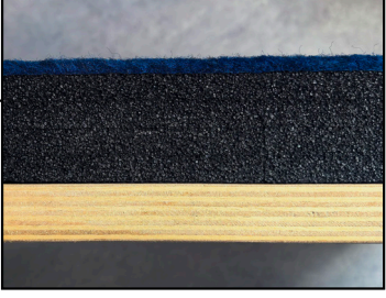
18mm plywood + 4.5cm carpet bonded foam
