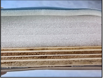
Platform Board: 18mm plywood + 5cm EPE + 0.5cm polyurethane foam, upholstered in 0.55mm PVC fabric
